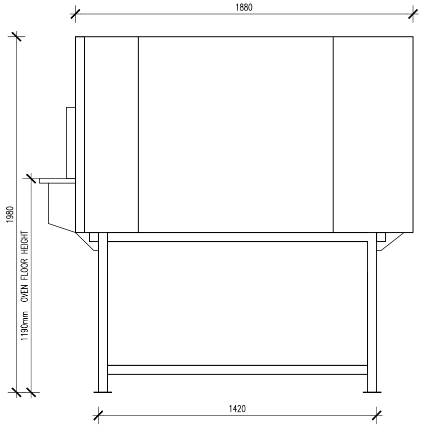
MODEL OT 120 X 160 SIDE VIEW
