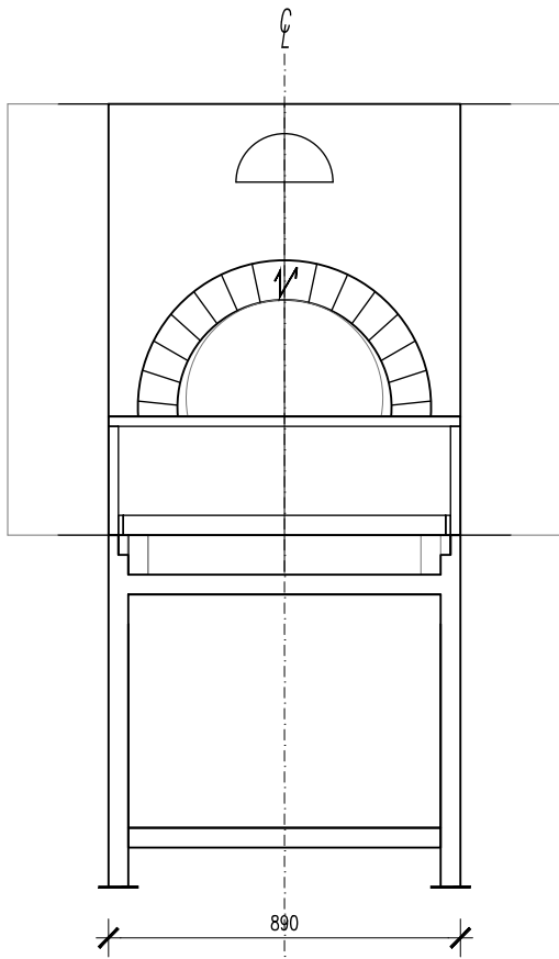
MODEL OT 120 X 160 FRONT VIEW
