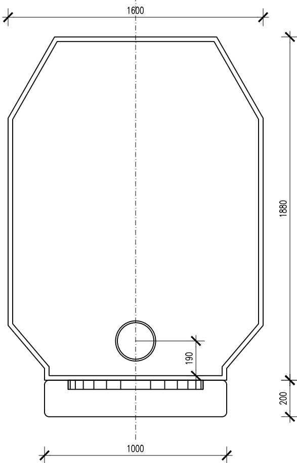
MODEL OT 120 X 160 PLAN VIEW
