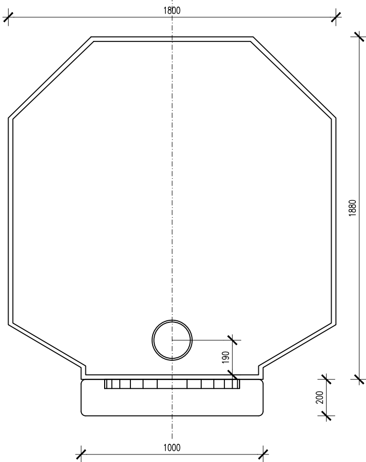
MODEL OT 140 X 160 PLAN VIEW
