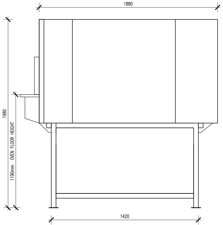
MODEL OT 140 X 160 SIDE VIEW
