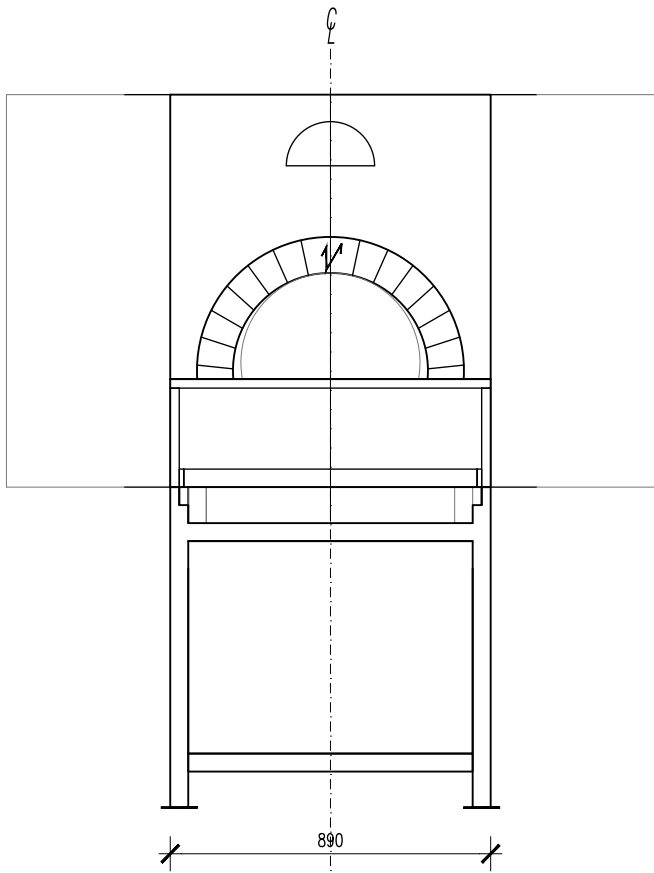
MODEL OT 140 X 160 FRONT VIEW
