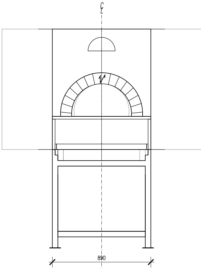
MODEL OT 140 X 180 FRONT VIEW
