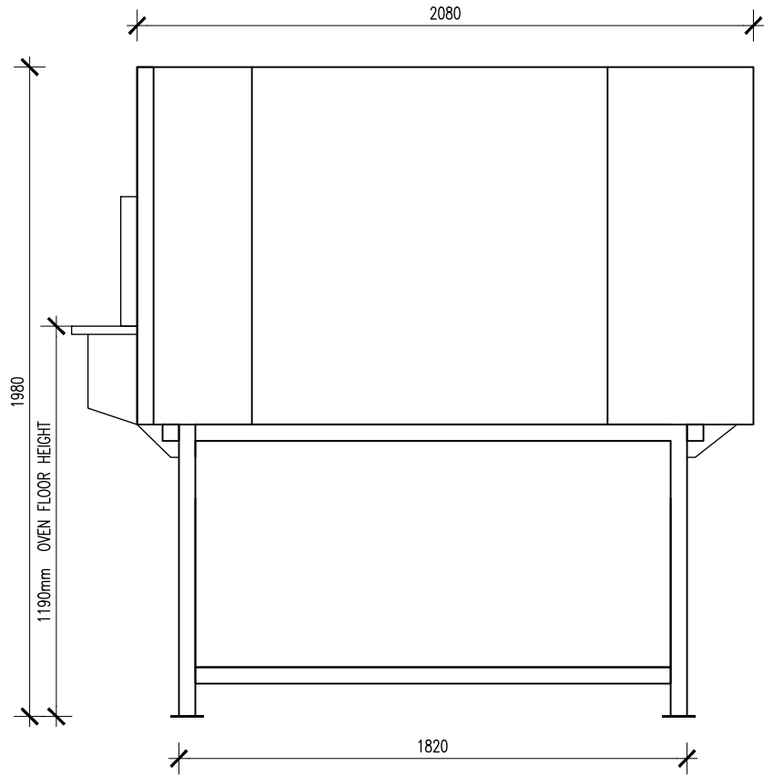
MODEL OT 140 X 180 SIDE VIEW
