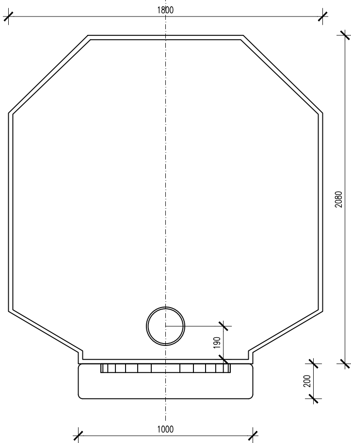
MODEL OT 140 X 180 PLAN VIEW
