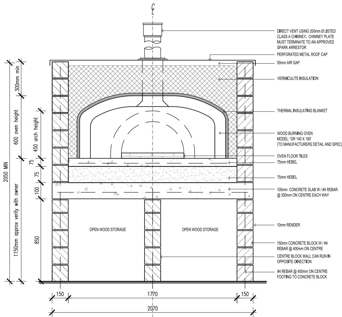
MODEL GR 140 X 180 FRONT VIEW
